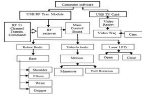
Fig.1 The general view of the mobile robot
