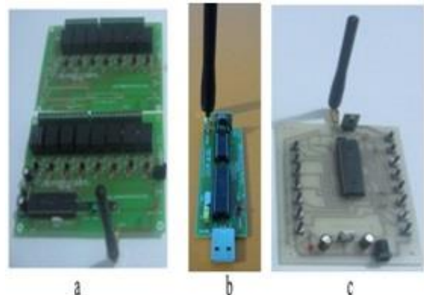
Fig.4 a) RF 15 channel main control receiver circuit card, b) RF 15 channel USB transmitter circuit, c) RF 15 channel transmitter command circuit
