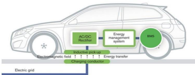
Fig 2.1 Static wireless EV charging
