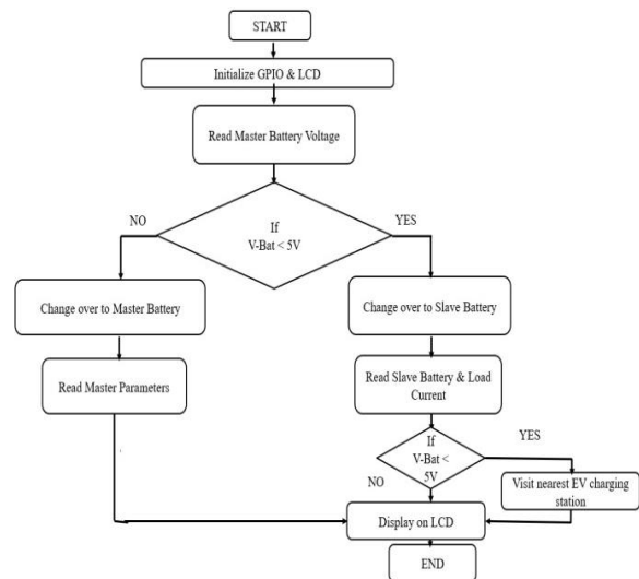
Fig 4.1 Flow Diagram
