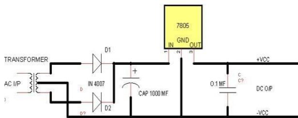
Figure 4.2.1 Power supply Circuit
