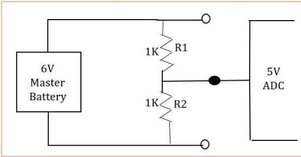
Fig 4.2 BMS of Master and Slave Battery
