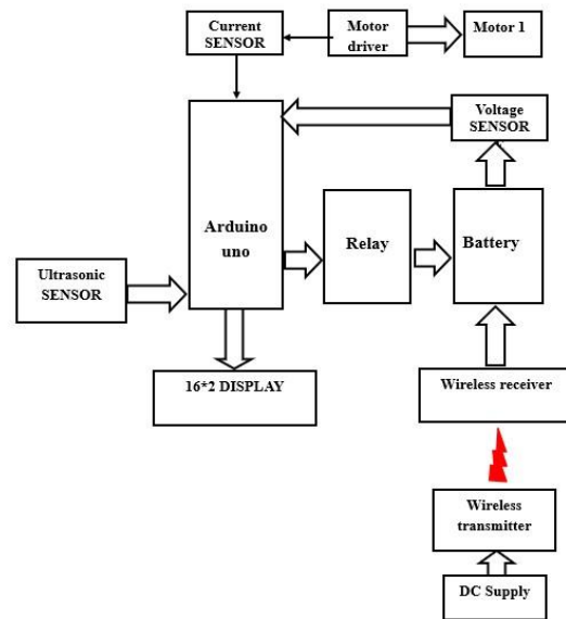
Fig 3.1 Block Diagram
