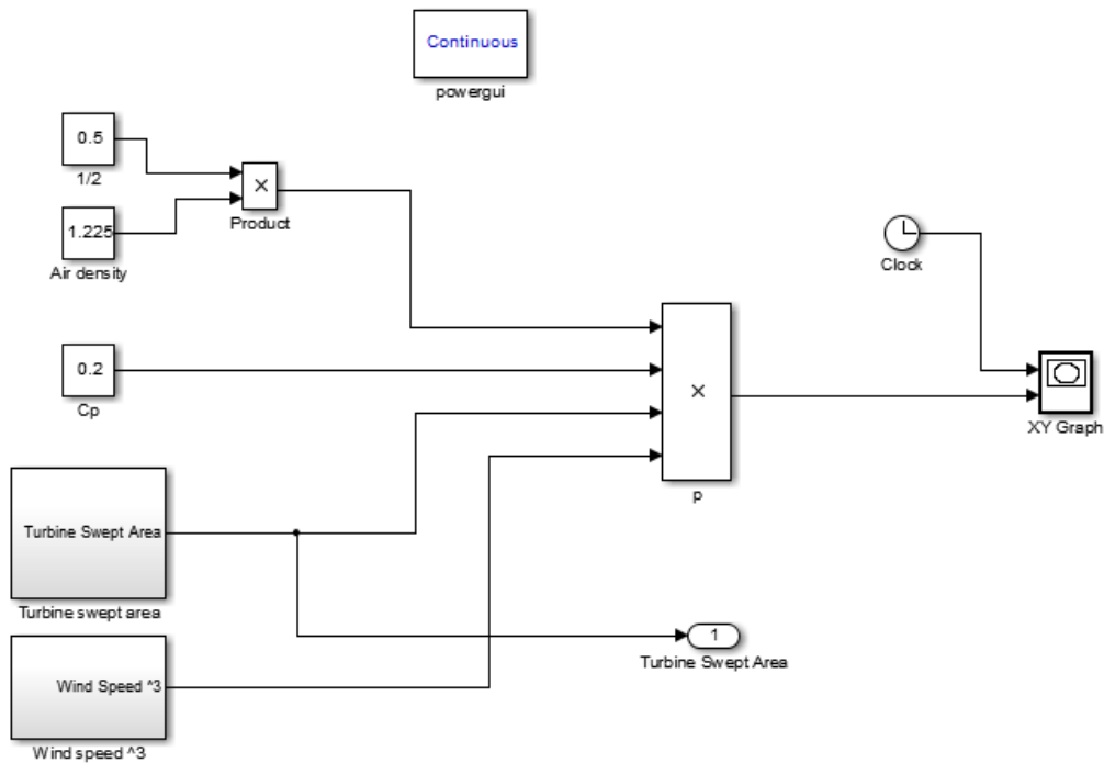
Figure 9. MATLAB Simulink model to calculate wind turbine output power.
