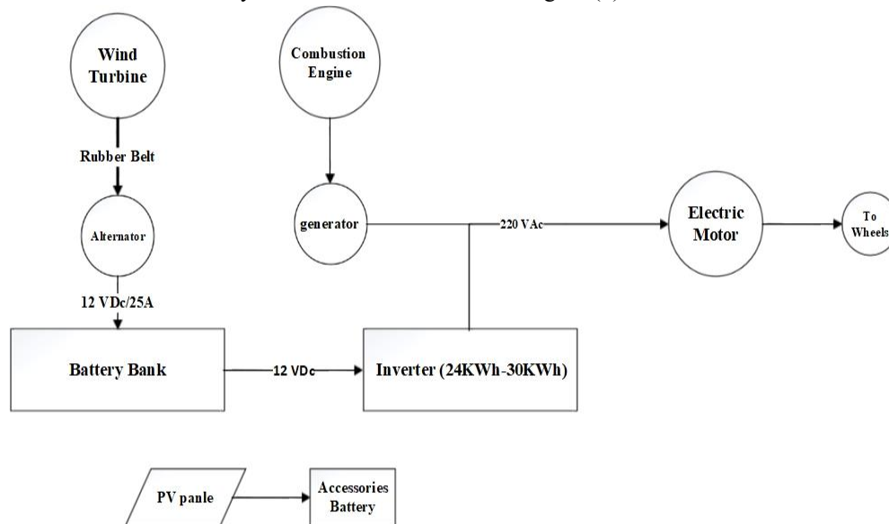
Figure 5. The studied model of hybrid vehicle.
