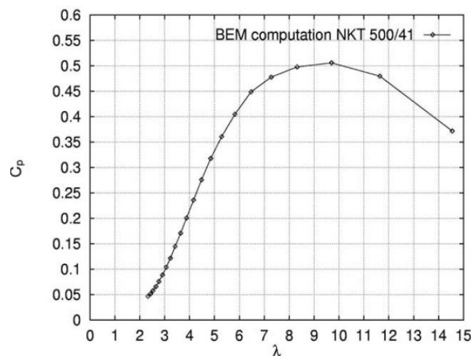
Figure 6. The relation between wind speed ratio and power efficiency factor.
