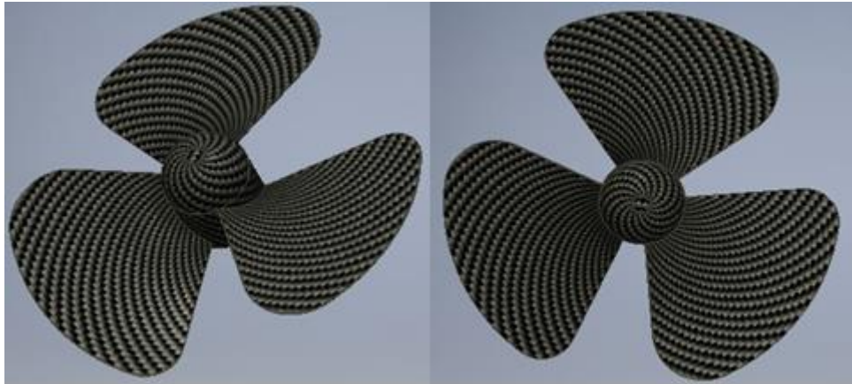
Figure 11. Wind Turbine Design using Autodesk Inventor.
