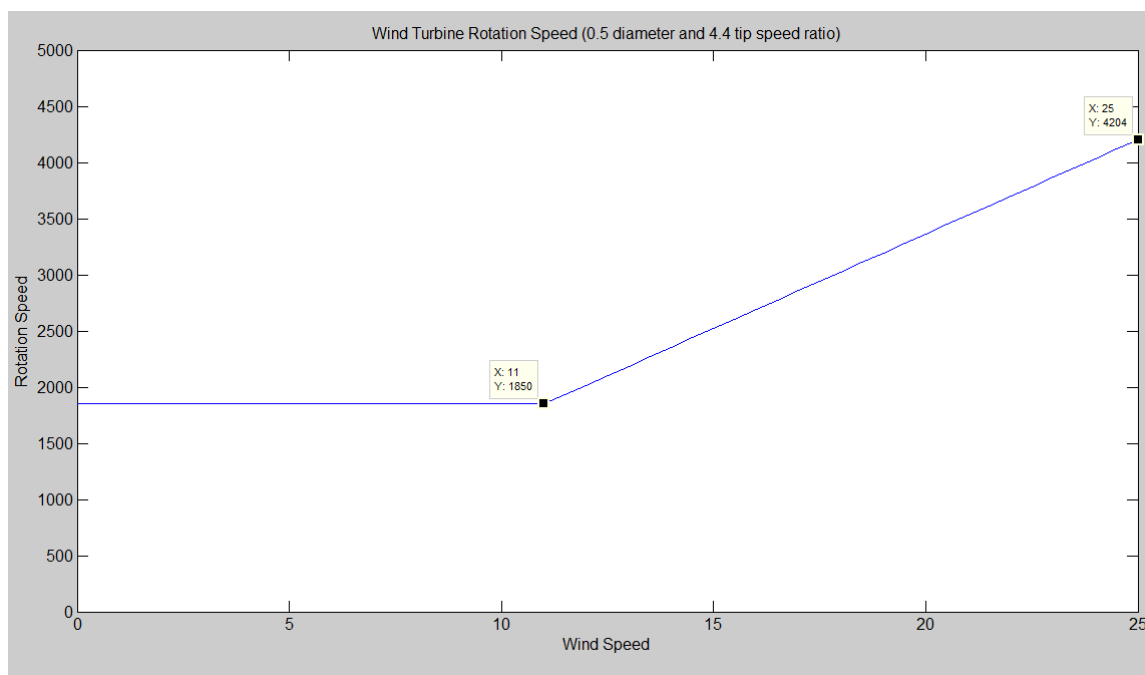
Figure 8. Wind turbine rotation speed for 0.5 diameter and 4.4 tip speed ratio.
