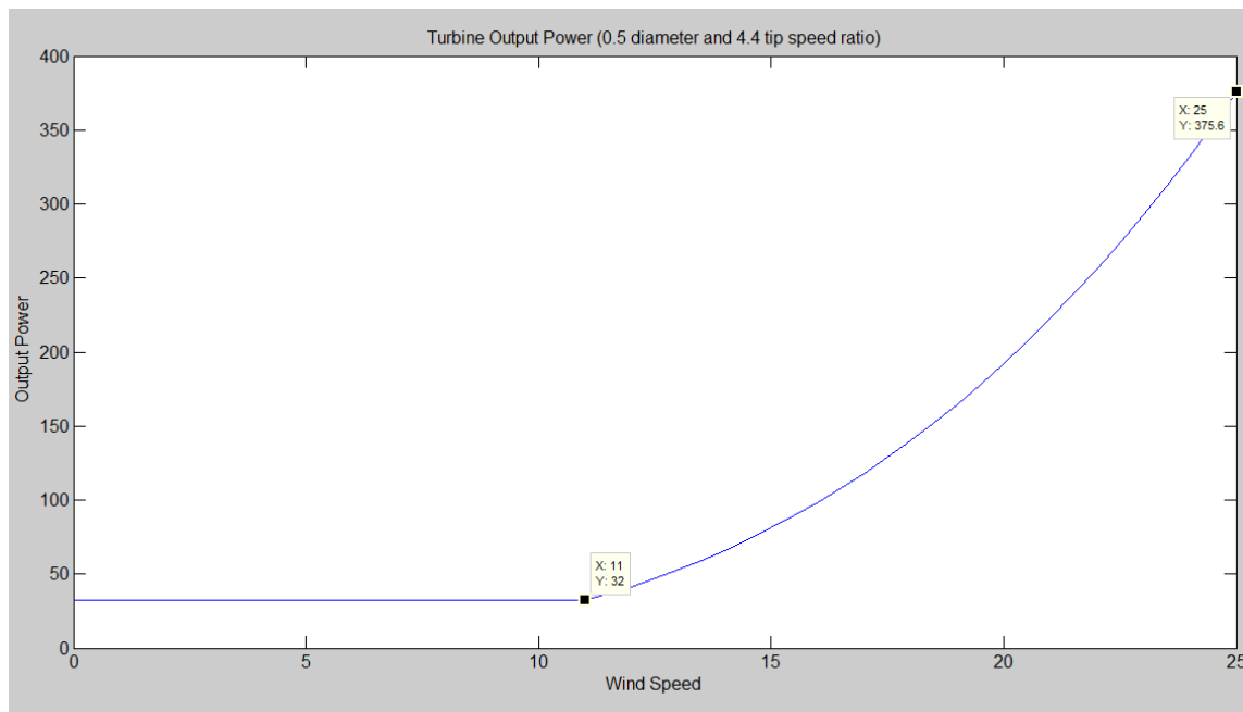
Figure 10. Wind turbine output power for 0.5 diameter and 4.4 tip speed ratio.
