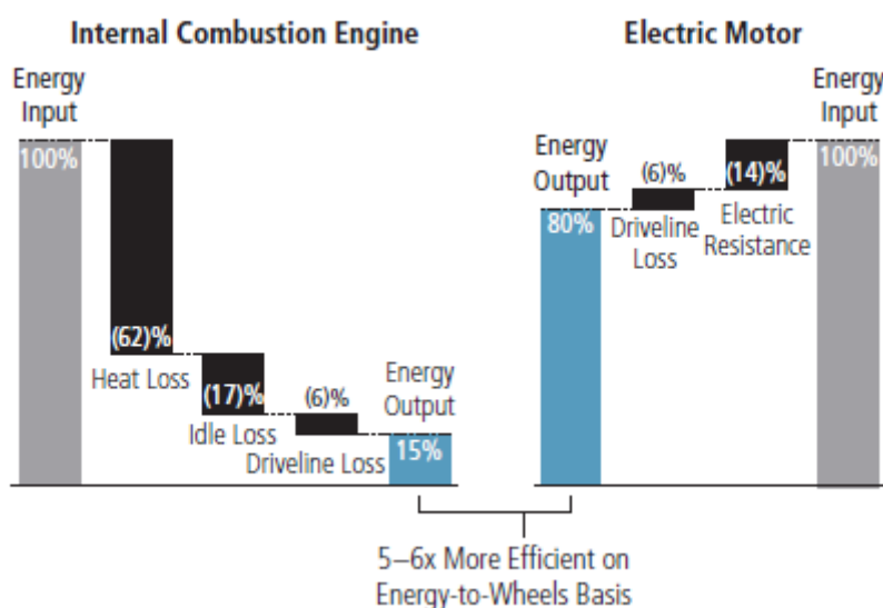
Figure 1. Electricity efficiency compared to combustion engines in powering cars.
