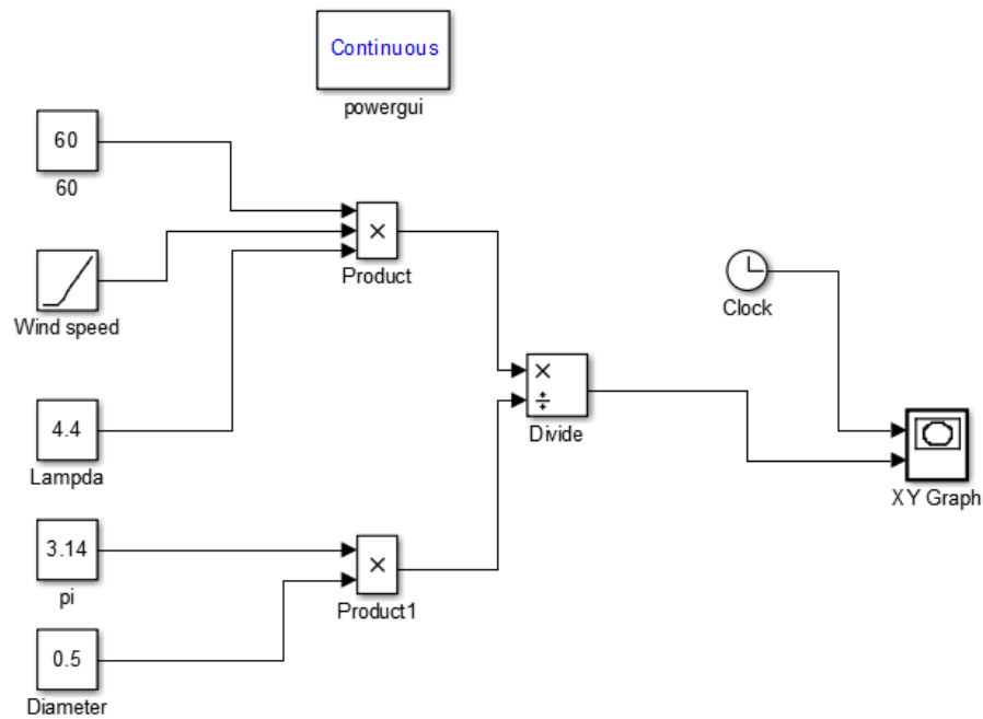
Figure 7. MATLAB Simulink model to calculate wind turbine rotation speed.
