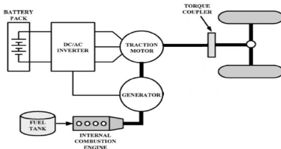
Figure 3. Series hybrid vehicles.
