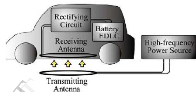
Figure 1: wireless car charging
