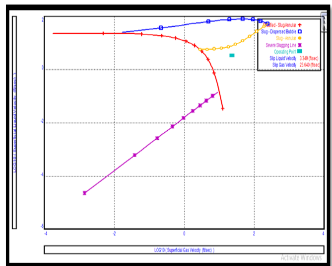
Fig. 10: A graph of Tie back – intermittent which indicate the operating point against the superficial gas and liquid velocity.
