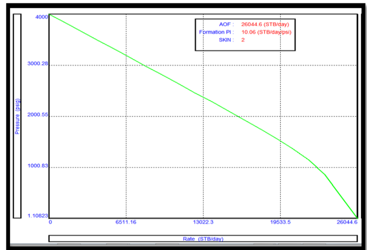
Fig. 2: Result of IPR Plot Darcy
