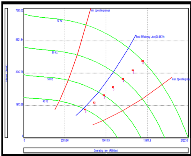
Fig. 7: Result of ESP Solution Plot
