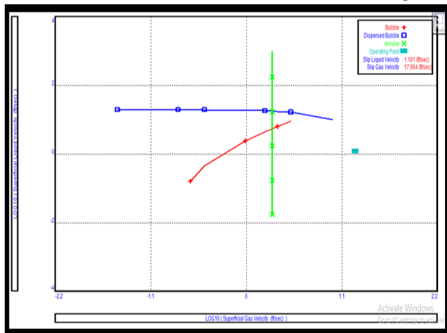
Fig. 8: A graph of Casing slug which indicate the operating point against the superficial gas and liquid velocity.
