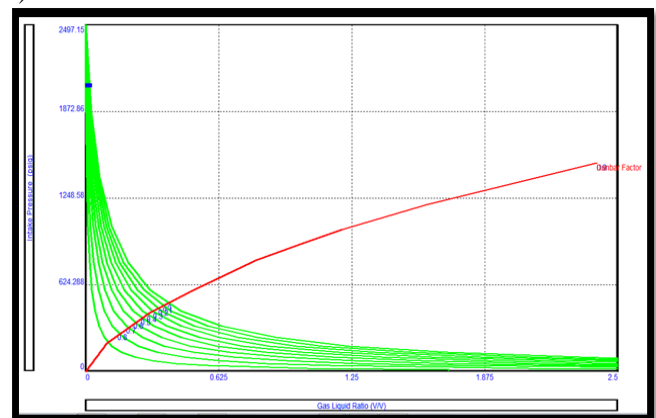
Fig. 3: Result of Gas Separation Sensitivity Plot
