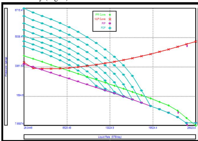
Fig. 5: Result of PDP vs. VLP Pressure Plot
