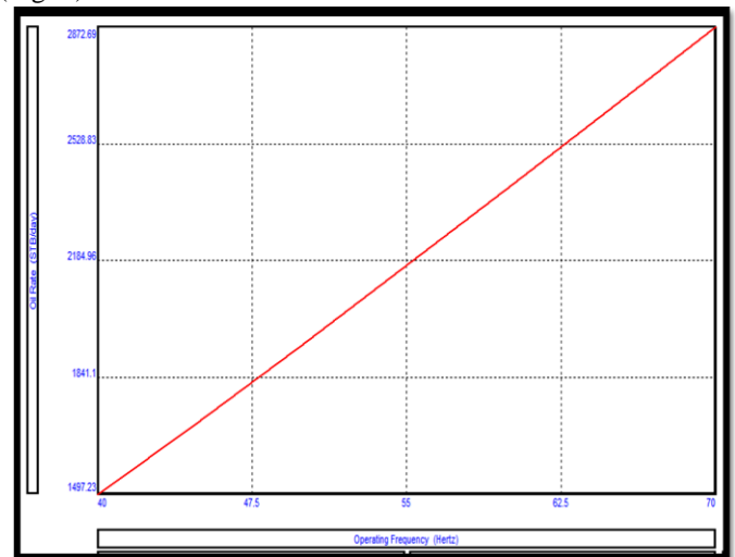
Fig. 6: Sensitivity Plot of Oil rate vs. Pump operating frequency
