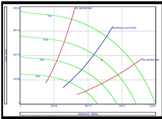
Fig. 4: Result of Pump Performance Curve
