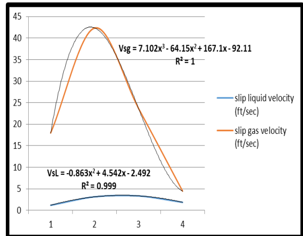
Fig. 12: Physic-Mathematical model
