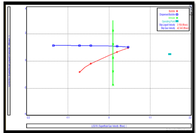
Fig. 9: A graph of Tubing slug which indicate the operating point against the superficial gas and liquid velocity.
