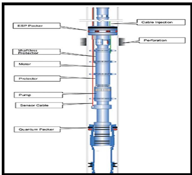
Fig. 1: Sketch showing the schematic for an Electrical Submersible Pump
