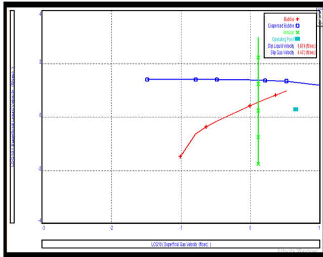
Fig. 11: A graph of Riser intermittent which indicate the operating point against the superficial gas and liquid velocity.
