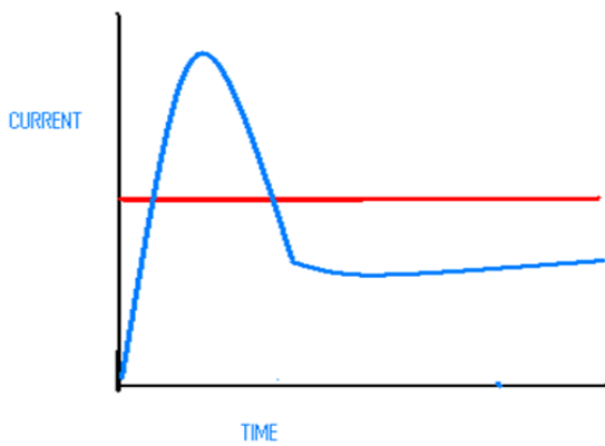
Figure 1: The blue line demonstrates the current in a typical strike [2], the red line shows the constant-current approximation used. The area beneath each graph (proportional to energy yield) is approximately equal. (Original source)
