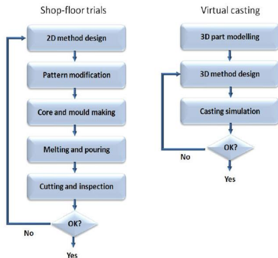
Figure 3. Comparison of conventional approach and integrated CAD/CAE/CAM approach
