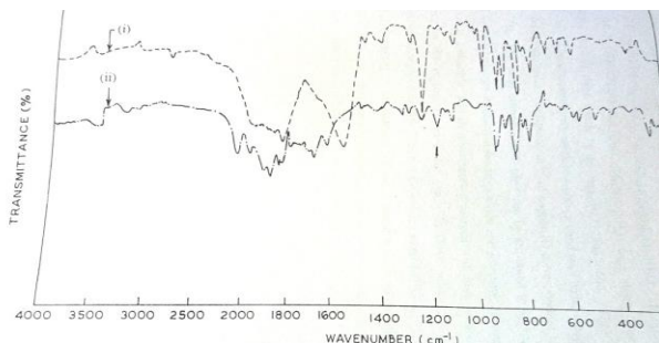
Fig. (3 A) IR SPECTRA OF ORGANIC COMPOUNDS (i) (C 10 H 10 N 3 O) (ii) (C 15 H 12 N 3 O)
