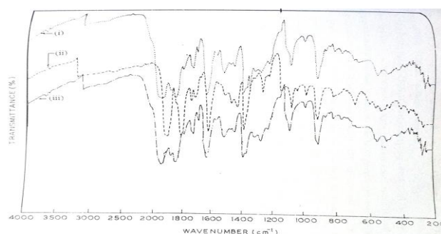
Fig. (3.1 A) IR SPECTRA OF COMPLEXES (i) [Co(C 10 H 10 N 3 O)]Cl (ii) [Co(C 10 H 10 N 3 O) 2 ]·2H 2 O (iii) [Co(C 15 H 12 N 3 O) 2 ]·2H 2 O
