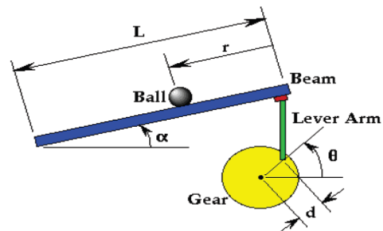
Figure 3 :- Ball and Beam system for mathematical analysis
