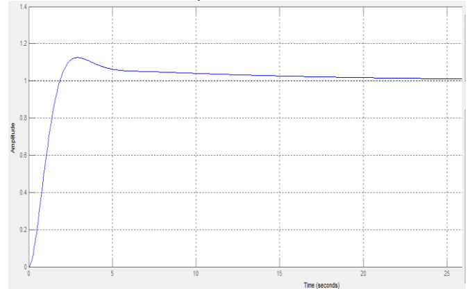
Figure 6:- Simulation results of Ball and Beam Model
