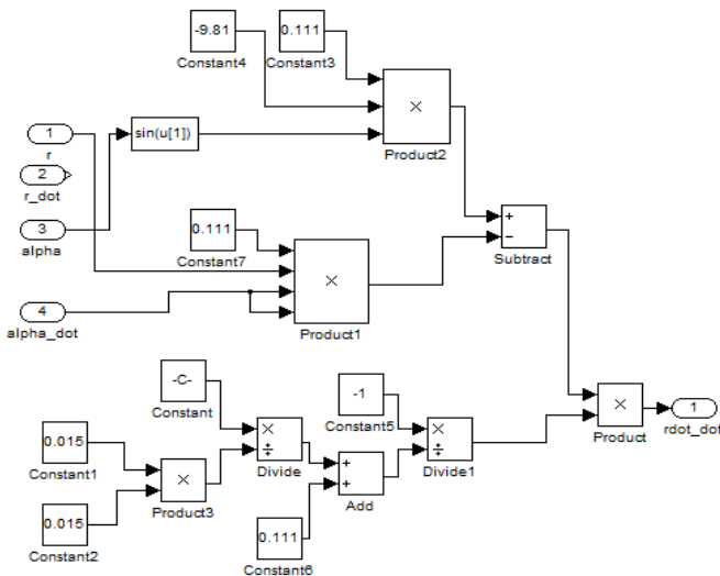
Figure 5:- Internal structure of Ball and Beam model
