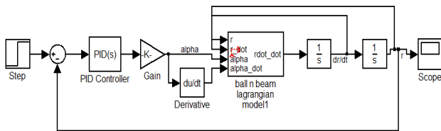
Figure 4:- Simulation model of Ball and Beam system
