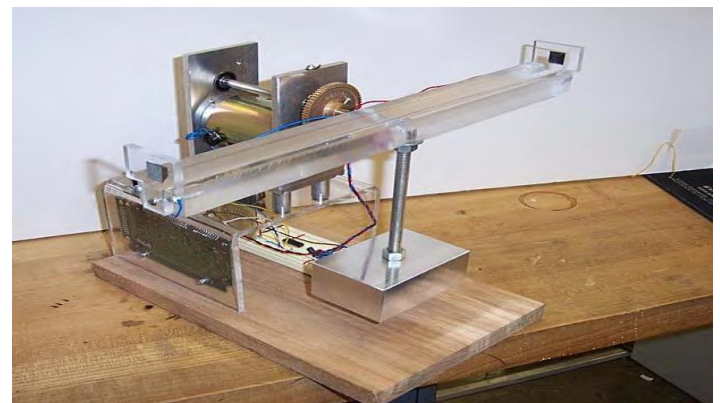
Figure .2:- Ball and Beam system model
