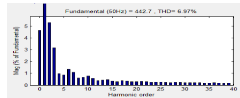
Fig.13 Output voltage of FFT level
