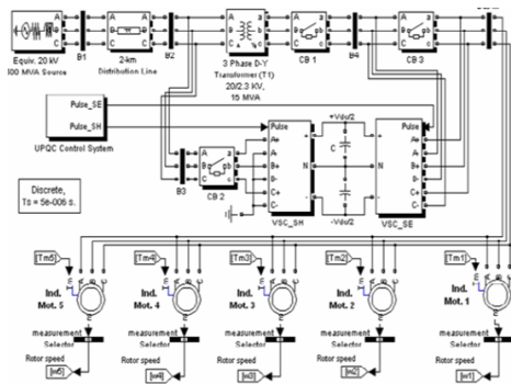
Fig.1 Common Shaft Induction Motors
