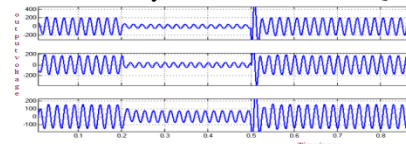
Fig 15 Waveform of Output current
