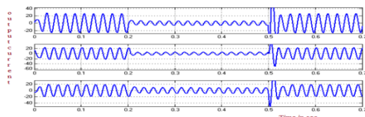
Fig.10 Waveform of Output current without controller
