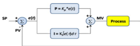
Fig.5. Block diagram of PI controller
