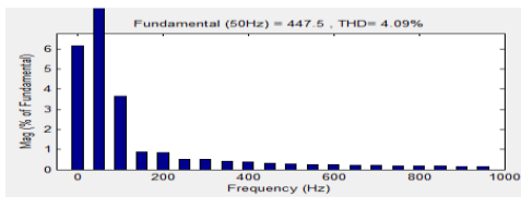
Figure:18 Output voltage of FFT level
