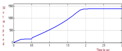
Fig.11 Waveform of Motor speed
