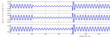
Fig.9 Waveform of output voltage of the system without controller
