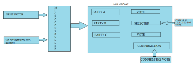
Figure 4. functional design of electronic voting system based on touch screen.
