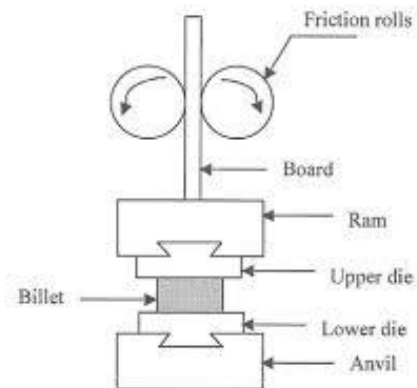
Figure 3: Mechanical board hammer
