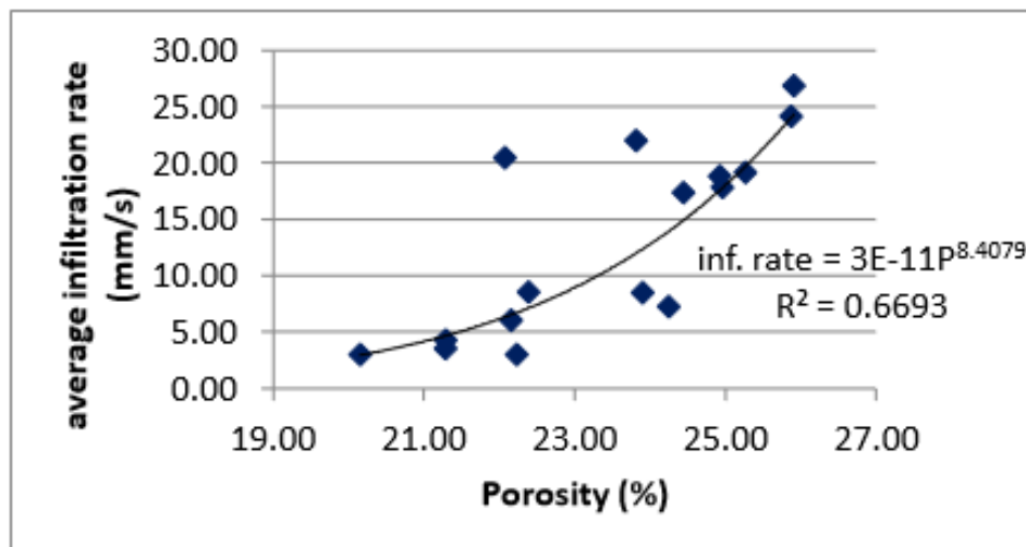
2.5 Infiltration rate VS porosity for sample of 10mm and 4.75mm
