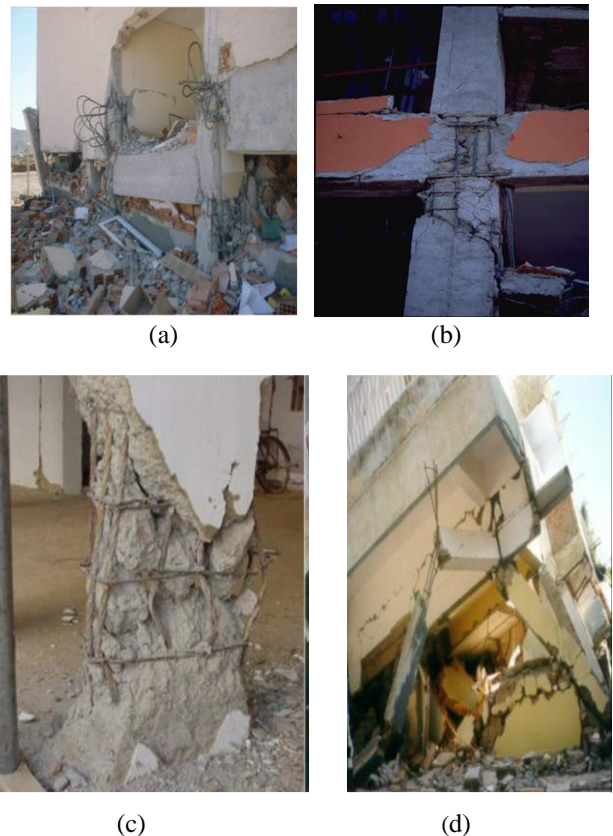
Fig 1.1 Failure of buildings due to storey mechanism in past earthquakes: (a) Failure of column with eccentric connection during Turkey earthquake, 2003 (b) failure of column and beam-column joint during Turkey earthquake, 2003 (c) and (d) Failure building due to column storey mechanism during Bhuj Earthquake, 2001.
