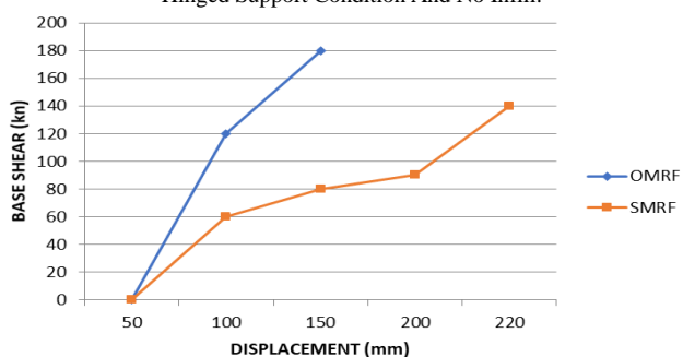
Fig 4.8 Shows The Pushover Curves Of 6S2B OMRF And 6S2B SMRF With Hinged Support Condition And No Infill.
