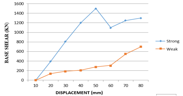
Fig.4.16 Showing The Comparison Of 6S4B SMRF Building With Strong And Weak Infill And Fixed Support Conditions.
