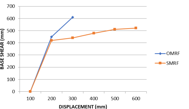
Fig 4.12 Shows The Pushover Curves Of 10S7B OMRF And 10S7B SMRF With Hinged Support Condition And No Infill.
