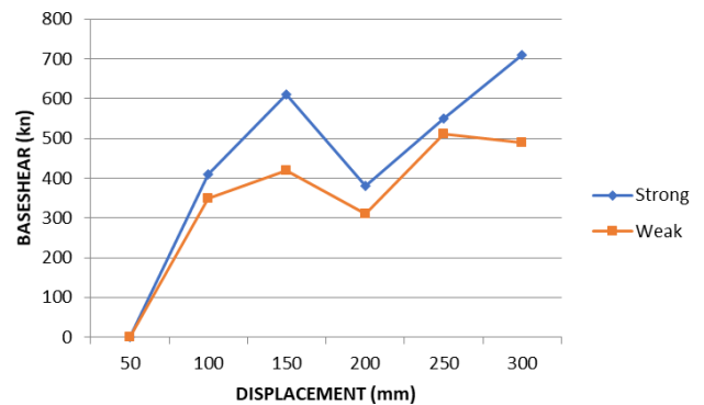
Fig.4.17 Showing The Comparison Of 6S2B SMRF Building With Strong And Weak Infill And Fixed Support Conditions.
