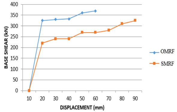
Fig 4.1 Shows The Pushover Curves Of 4S7B OMRF And 4S7B SMRF With Fixed Support Condition And No Infill.
