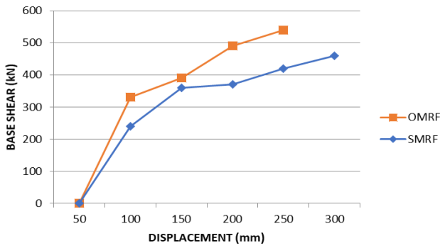
Fig 4.5 Shows The Pushover Curves Of 8S7B OMRF And 8S7B SMRF With Fixed Support Condition And No Infill
