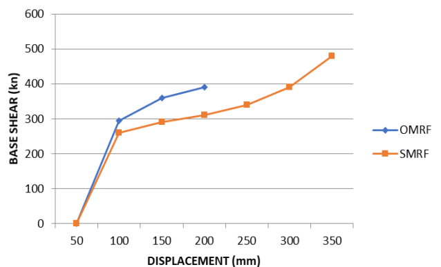
Fig 4.4 Shows The Pushover Curves Of 6S6B OMRF And 6S6B SMRF With Fixed Support Condition And No Infill.
