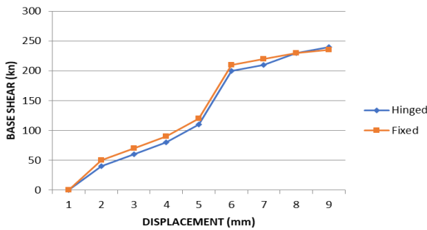
Fig 4.13 Shows The Pushover Curves Of 6S4B SMRF With Both Fixed And Hinged Support Condition And No Infill.
