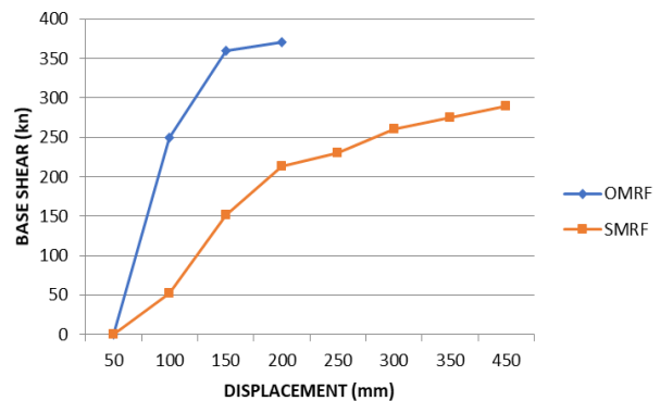
Fig 4.3 Shows The Pushover Curves Of 6S4B OMRF And 6S4B SMRF With Fixed Support Condition And No Infill.
