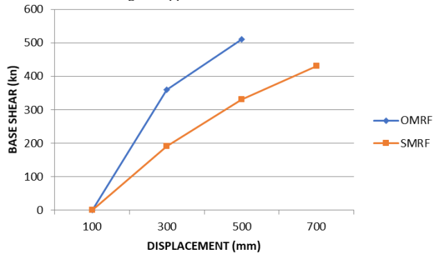
Fig 4.11 Shows The Pushover Curves Of 8S7B OMRF And 8S7B SMRF With Hinged Support Condition And No Infill.
