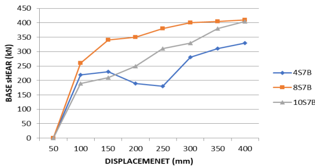
Fig.4.14 Showing The Storey Wise Comparison Of SMRF Buildings With Fixed Support Conditions And No Infill.
