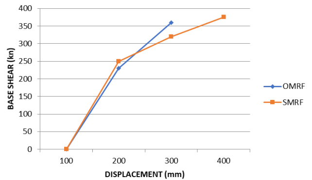
Fig 4.10 Shows The Pushover Curves Of 6S6B OMRF And 6S6B SMRF With Hinged Support Condition And No Infill.
