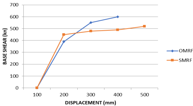
Fig 4.6 Shows The Pushover Curves Of 10S7B OMRF And 10S7B SMRF With Fixed Support Condition And No Infill
