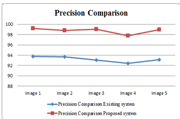
Fig. 7: Precision Comparison
