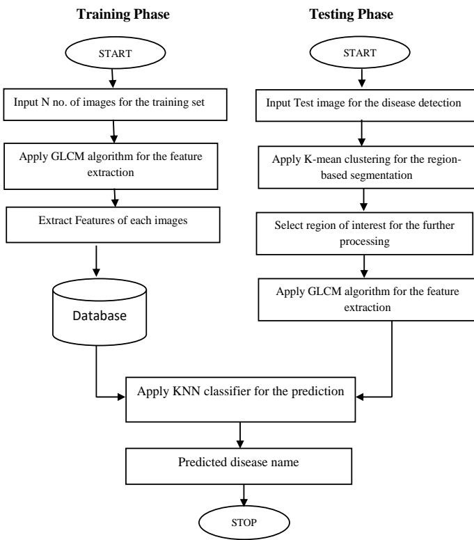
Fig. 1: Proposed Flowchart
