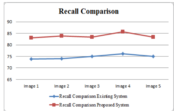
Fig. 8: Recall Comparison
