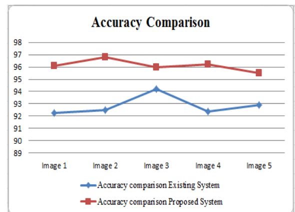
Fig. 9: Accuracy Comparison
