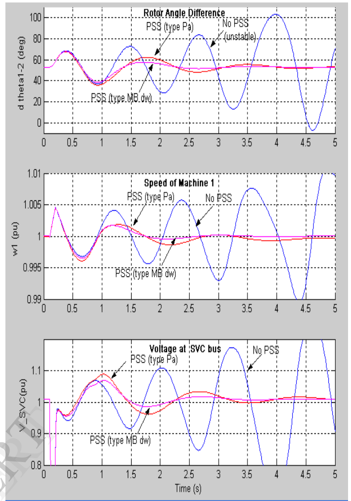
Figure 7. Impact of single band and multiband power system stabilizer
