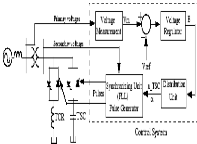
Figure1: Single-line Diagram of an SVC along with Its Control System Block
