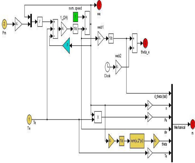
Figure-5: Mechanical Parts of a three phase synchronous Machine
