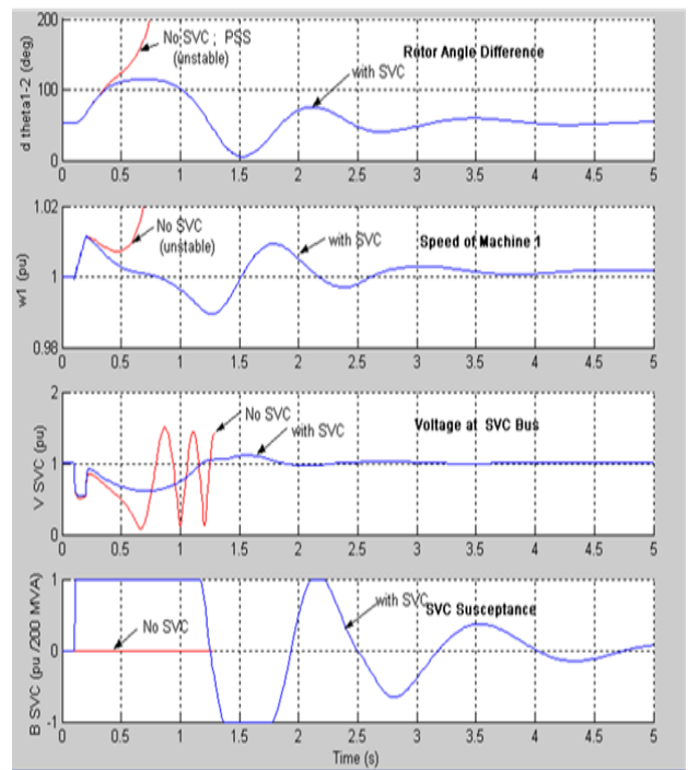
Figure 8: Comparison of results of a 6 cycle 3 phase Fault when PSS in service and with and without SVC
