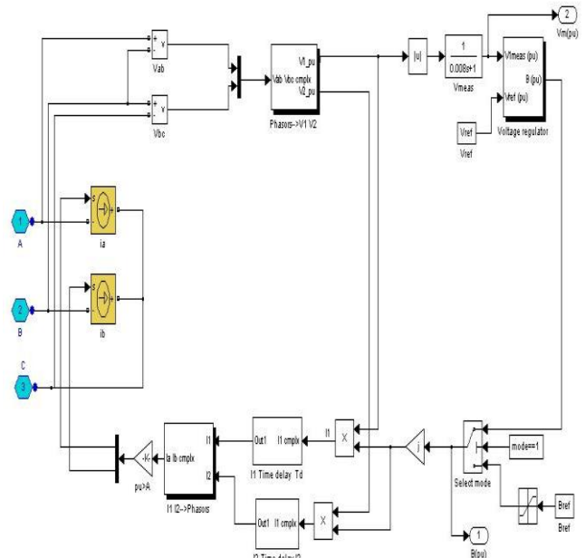
Figure 4: Two machine SVC/PSS subsystem
