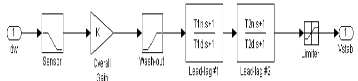
Figure 2: The Generic Power System Stabilizer
