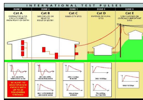
Figure 3. Surge current waves according to the recent international standards.
