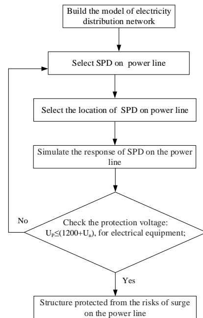
Figure 2. Selection steps of SPD on the power line.
