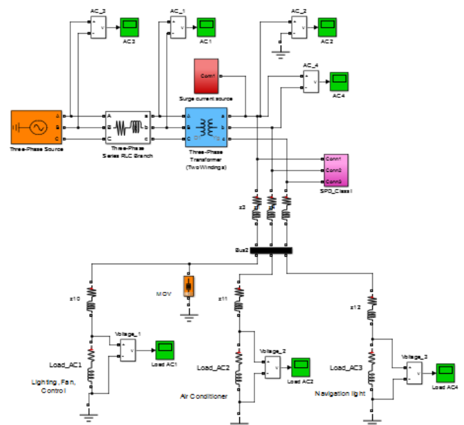
Figure 4. Power distribution network simulation diagram in Matlab.
