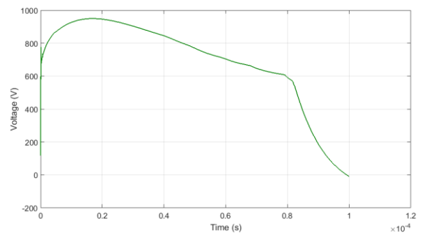
Figure 6. Protection voltage waveform at load when surge current 8/20\mu\text{s} 40kA propagates on the power line after the transformer goes into the SMSB, with the SPD 275V-100kA installed in the EMSB and the SPD 275V- 70kA in the MSB.
