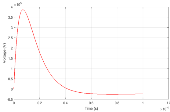
Figure 5. Protection voltage waveform across the load when SPD is not installed.
