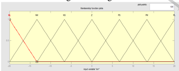
Fig 13: Membership functions for error input
