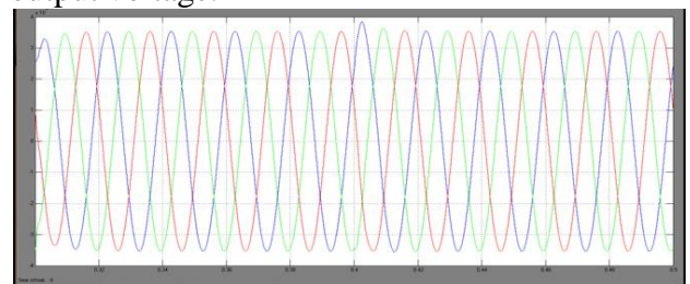
Fig.10: Load Voltage (PCC voltage) waveforms with DSTATCOM
