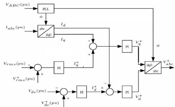
Fig.5 Block Diagram of DSTATCOM Control
