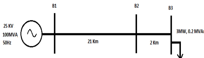
Fig.6:Test system
