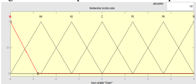
Fig. 14 Membership functions for change in error input
