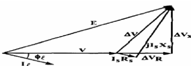
Fig. 3 Phasor diagram for uncompensated
