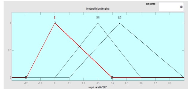
Fig 16 Output membership functions for change in K_i
