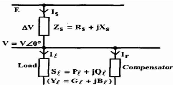
Fig. 2 A Simple Circuit for demonstrating the voltage regulation principle.
