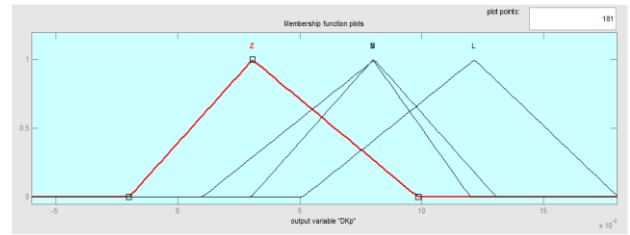
Fig 15 Output membership functions for Change in K_p
