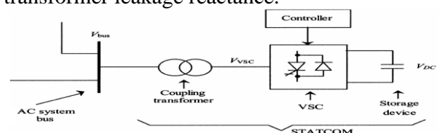
Fig.1. Block Diagram of the voltage source converter based DSTATCOM
