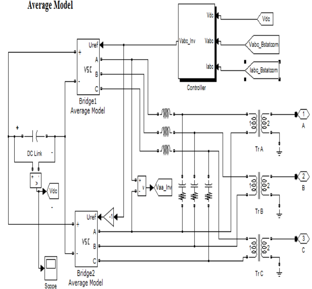
Fig. 9: Simulink model of DSTATCOM
