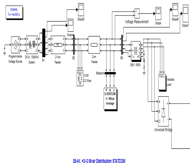
Fig.8: Simulink model with DSTATCOM
