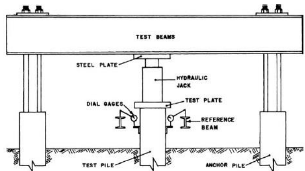
FIGURE : 3 LOAD TEST ON SINGLE PILE
