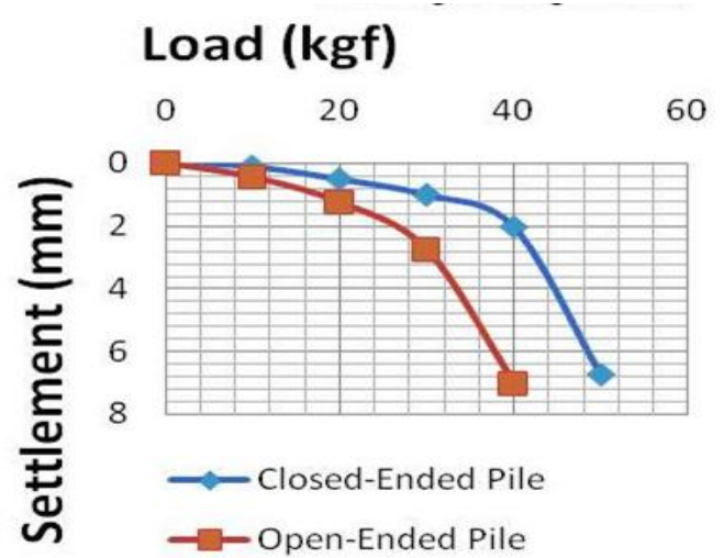
FIGURE : 2 PILE TEST ON SOIL STARTA FOR BEARING CAPACITY
