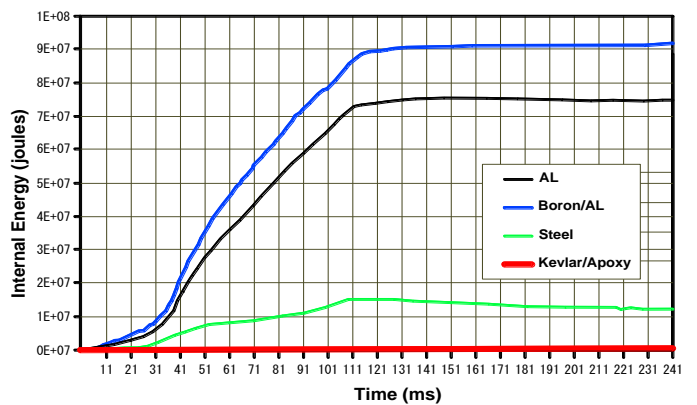
Fig. (14) Internal energy of all parts due to material changing.
