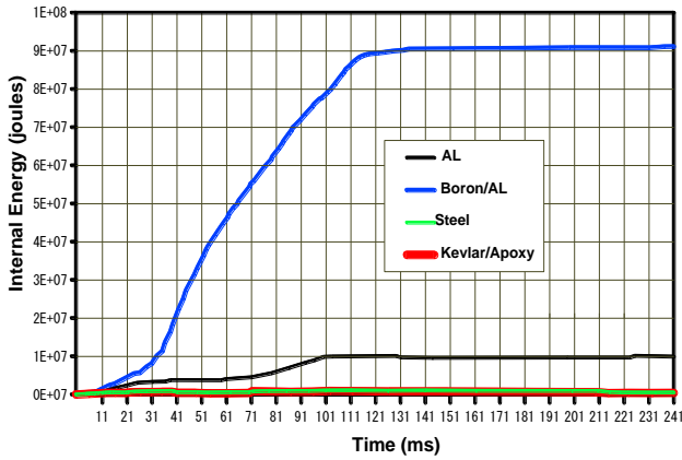
Fig. (8) Internal energy of bumper due to material changing
