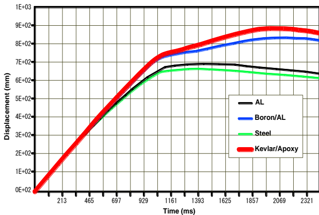
Fig. (3) Displacement of node 16154 due to frame material changing
