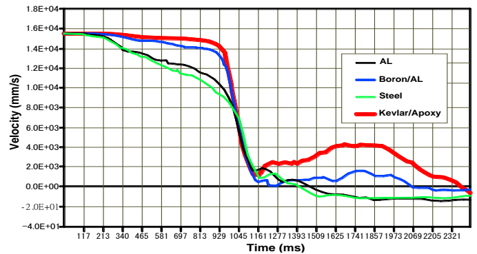
Fig. (13) Velocity of node 16154 due to all parts material changing.
