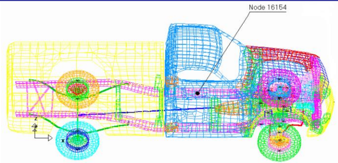
Fig. (1). Position of the node 16154 on the model.
