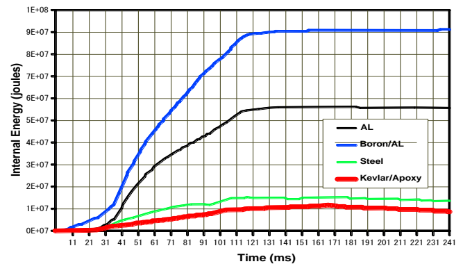
Fig. (5) Internal energy of frame due to material changing.
