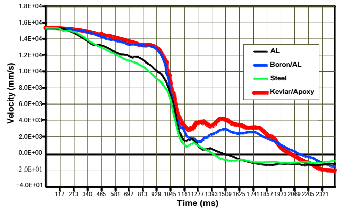
Fig. (4) Velocity of node 16154 due to frame material changing.
