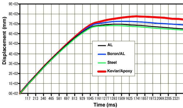
Fig. (9) Displacement of node 16154 due to hood, fenders, wheel housing and doors material changing.
