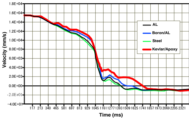
Fig. (10) Velocity of node 16154 due to hood, fenders, wheel housing and doors material changing.
