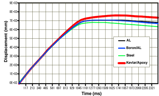
Fig. (6) Displacement of node 16154 due to bumper material changing.
