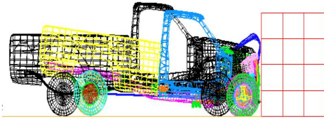
Fig. (2) Vehicle before and after the frontal impact test [1].
