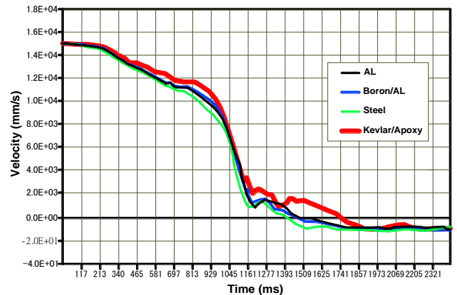
Fig. (7) Velocity of node 16154 due to bumper material changing.
