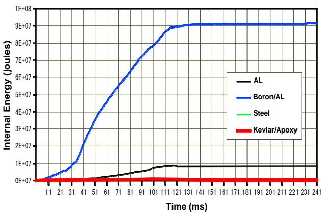
Fig. (11) Internal energy of hood, fenders, wheel housing and doors due to material changing
