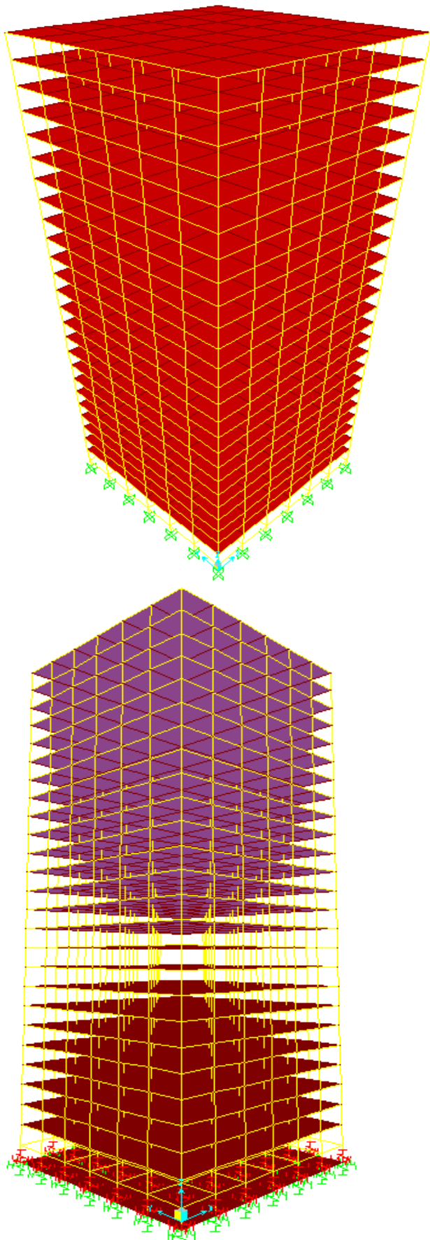
Fig: 2 Fixed base 3D model and Winkler 3D model for Raft foundation (0.8m, 1m, 1.2m)
