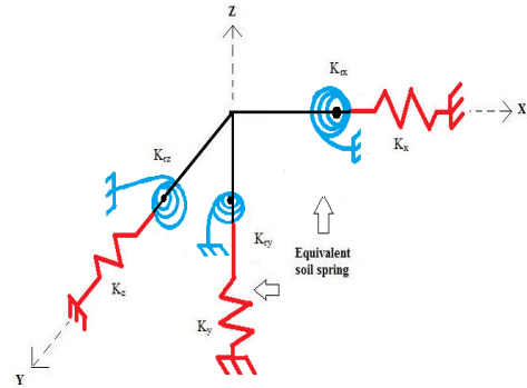
Fig: 1 Equivalent Spring Stiffness.
