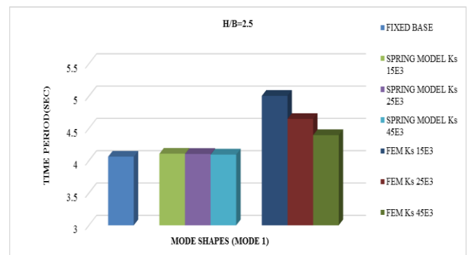
Fig: 4 show the variation of time period of fixed base, spring model and FEM model for 25floors.
