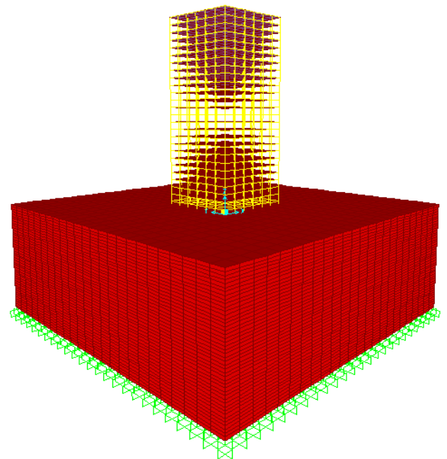
Fig: 3 3D elastic continuum (FEM) models for different types of soil (Soil media: 120mx120mx45m).
