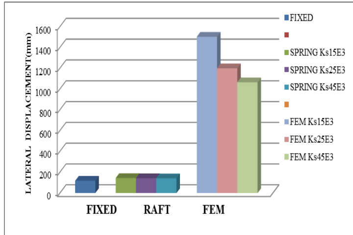
Fig: 6 show the variation of lateral displacement of fixed base, spring model and FEM model for 25 floors.
