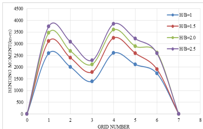
Fig: 6 show the variation of Bending Moment in Y-Y direction for 10, 15, 20 and 25 floors.
