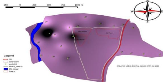
Fig. 6: Spatial variation map of Sulphate
