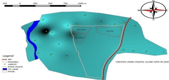
Fig. 2: Spatial variation map of Chloride
