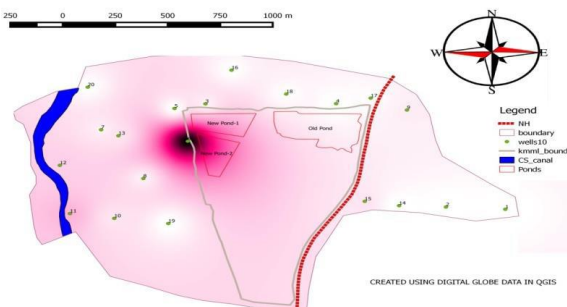
Fig. 4: Spatial variation map of Iron
