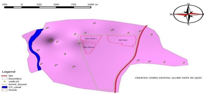
Fig. 3: Spatial variation map of Hardness
