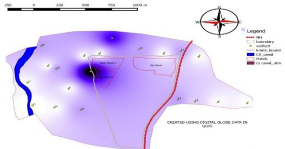
Fig. 5: Spatial variation map of pH
