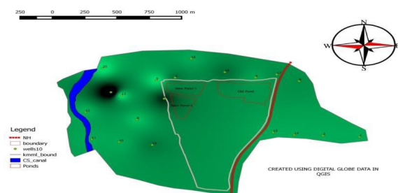
Fig. 2: Spatial variation map of Alkalinity
