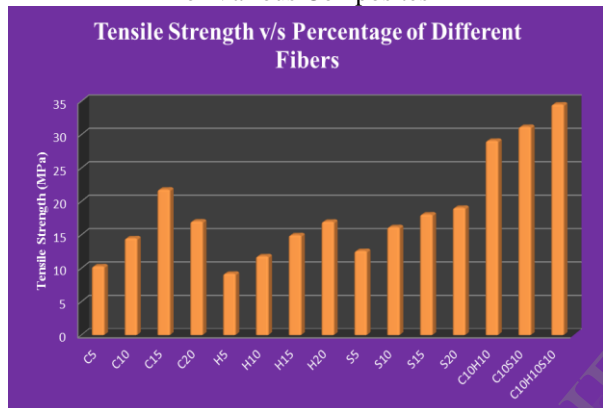
Figure 3: Comparative Bar Chart of Tensile Strength of Various Composites
