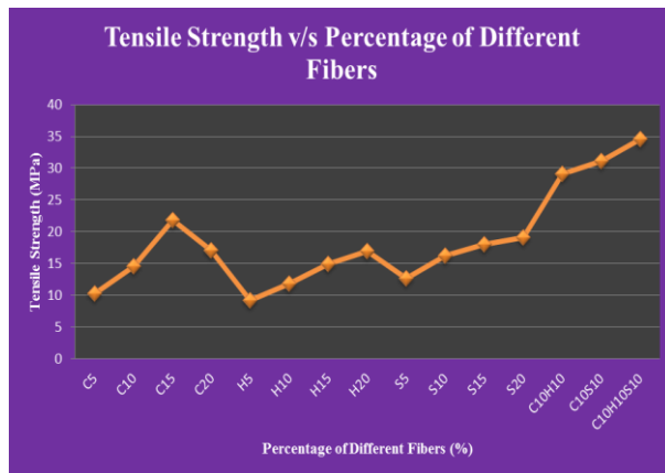
Figure 3: Comparative Line Chart of Tensile Strength of Various Composites
