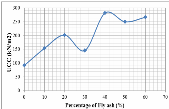
Fig 3 Variation in UCC with the Addition of Varying Percentage of Fly Ash
