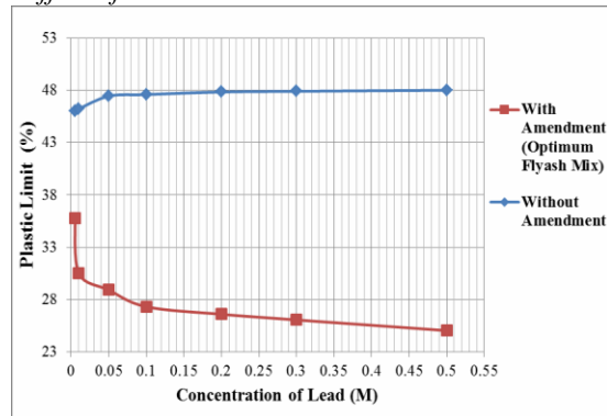
Fig 5 Variation of Plastic Limit on Contaminated CH Clay Due to Addition of Amendment
