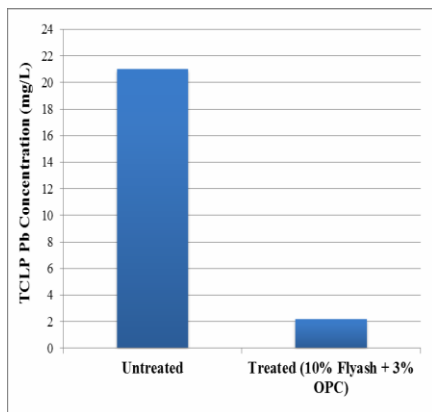
Fig 7 TCLP Pb concentration of untreated (control) and treated samples
