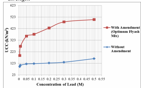
Fig 6 Variation of UCC on contaminated CH clay due to addition of amendment
