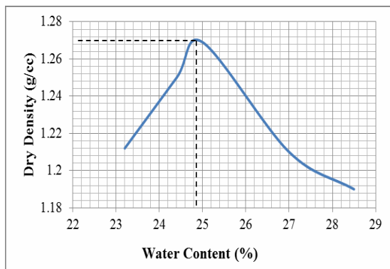
Fig 4 Compaction curve of Bentonite + Optimum mix
