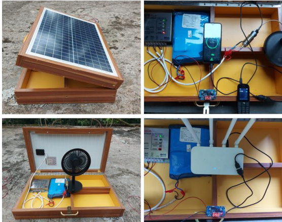
Fig. 3. Solar powered portable charging unit [18]
