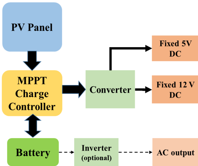
Fig. 1. Block diagram of general system configuration
