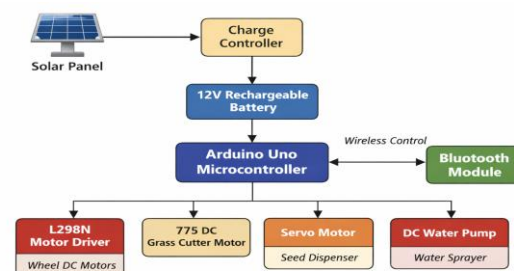
Fig. 2: System Architecture of Solar Power Multi-Purpose Agri Bot
