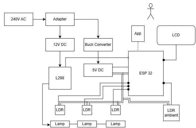
Figure 3: Block Diagram
