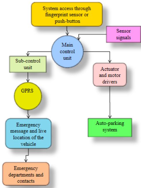
Fig. 1) Functional Block diagram of the designed system.
