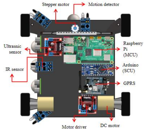
Fig. 2) Car prototype with equipment.
