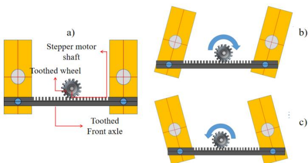
Fig. 3) Steering action using stepper motor.
