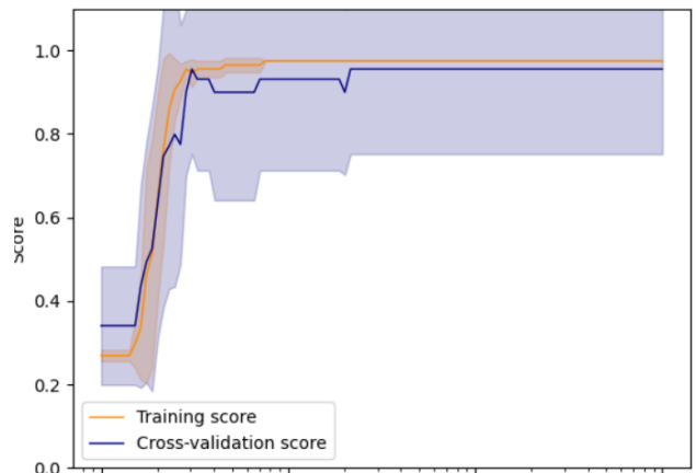
Figure IV.1 SVM Validation
