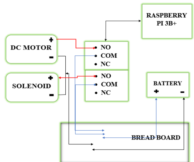
Fig 11: Circuit diagram for solenoid operation
