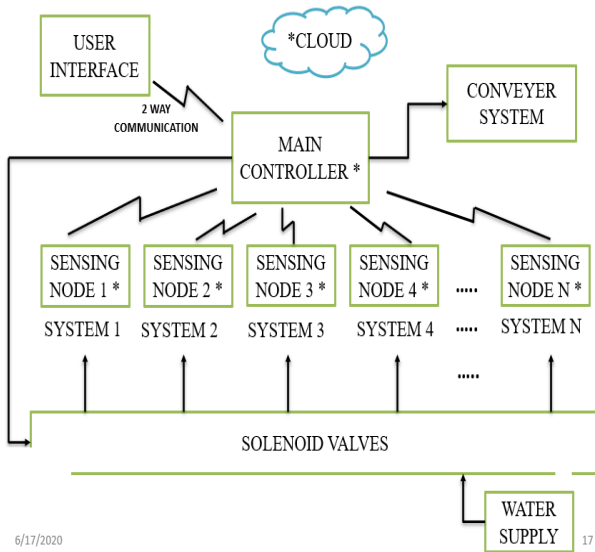
Fig 8: IoT system Block Diagram
