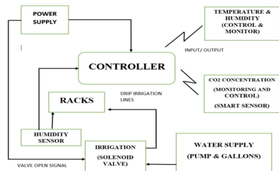
Fig 2: Sensing Node block diagram
