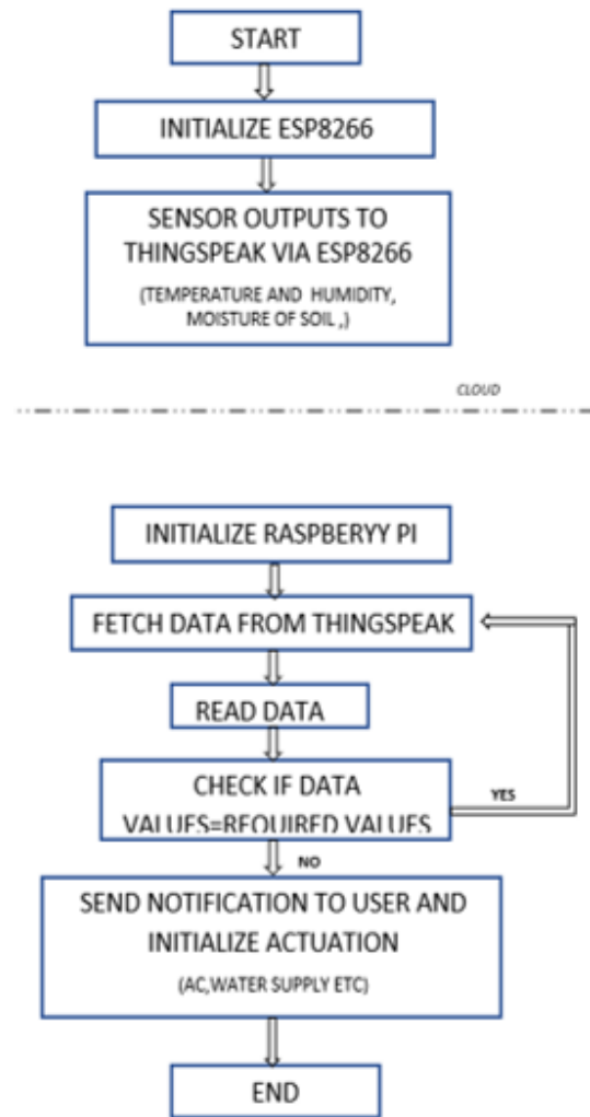
Fig7: Flow Diagram of the working of the sensing Node and Storing the value to the cloud.
