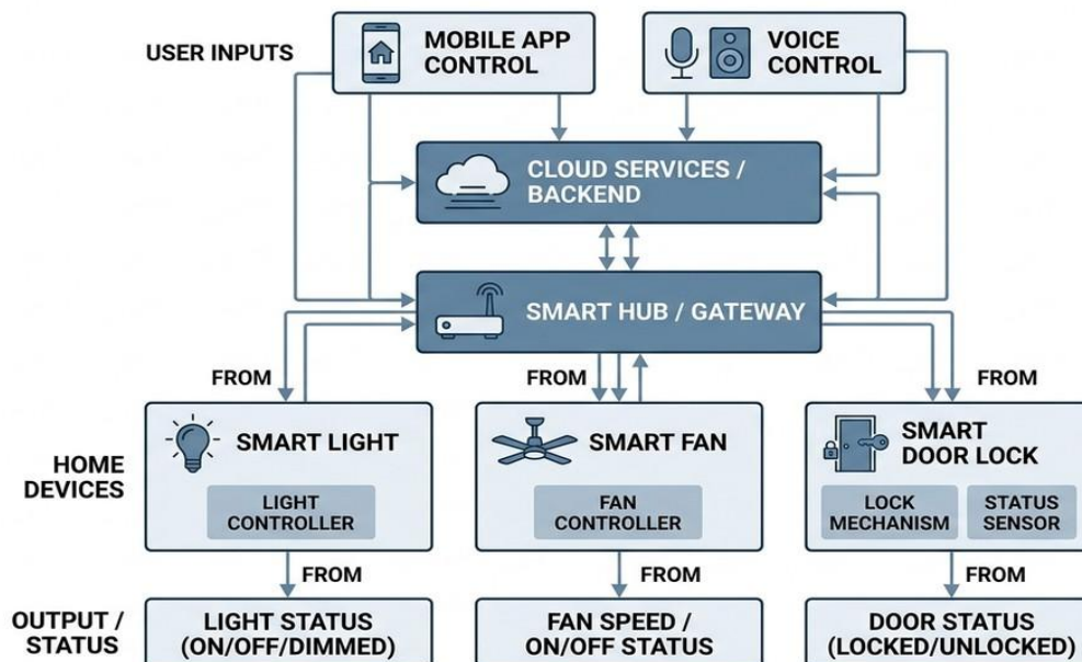
Fig. 1: Block diagram of mobile and voice controlled smart switch for home automation.
