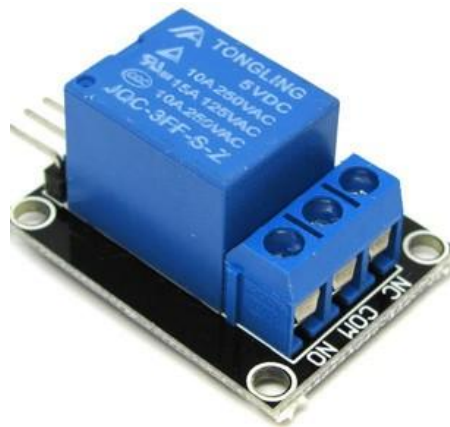
Fig. 3: Relay.
