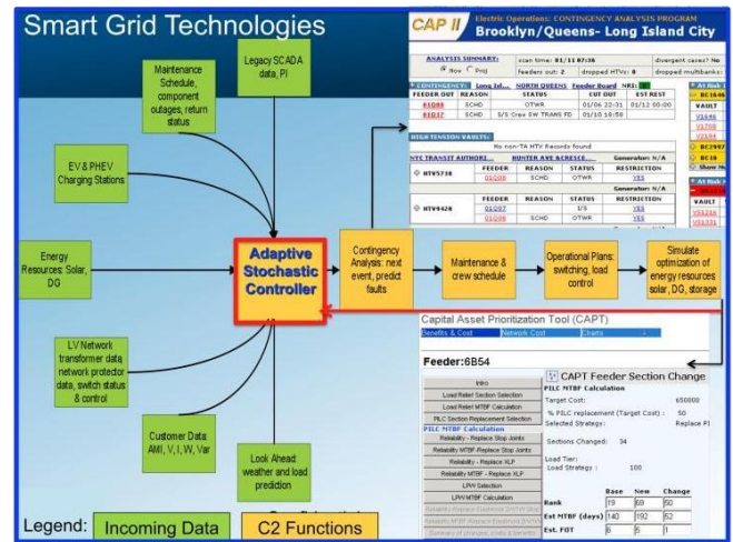
Figure 6. The Smart Grid must optimally interpret incoming data from many new sources (green) with new controls such as Contingency Analysis Programs (CAP in the upper right) and Capital Asset Prioritization Tools (CAPT in lower right).
