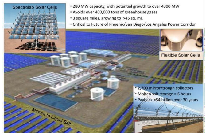
Figure 4. An artist's representation of the first 280 MW module of a Solar Thermal Power Plant complex southwest of Phoenix, Arizona, that will be selling power into the Western Interconnect and Southern California (image courtesy of Arizona State University).
