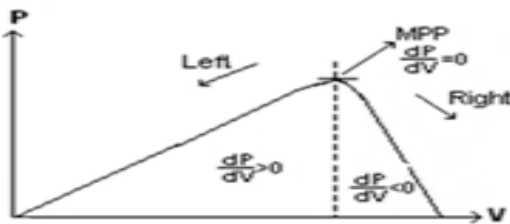
Fig. 2: Basic idea of incremental conductance method on a P-V Curve of solar module
