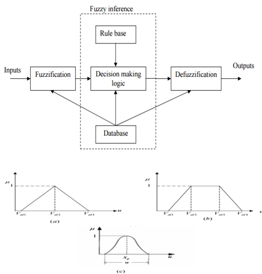
Fig. 5: (a) Triangle, (b) Trapezoid, and (c) Bell membership functions.
