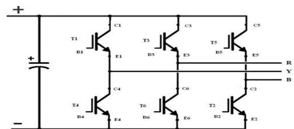
Fig. 4: Three phase inverter
