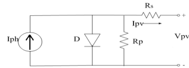
Fig. 3: Equivalent Circuit
