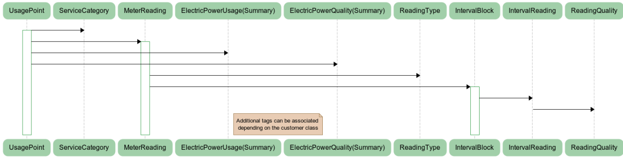
Fig. 1. Sequence diagram of energy usage information (XML) represented through green button standard
