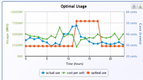
Fig. 10. Interface of manage peak usage
