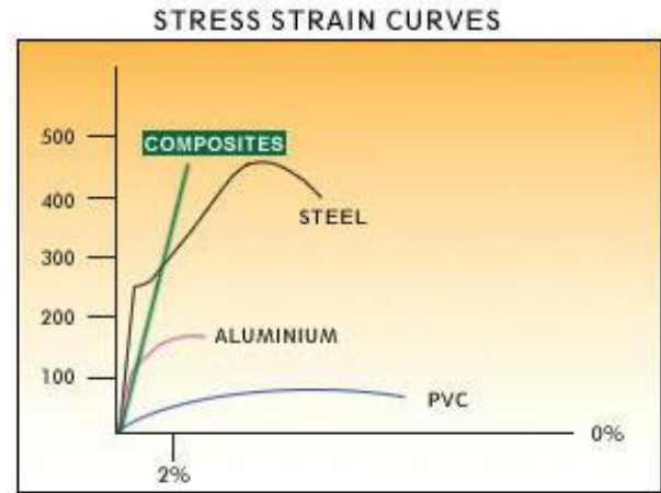
Graph 1: Schematic Diagram of stress vs strain with respect to behavior of Composites in comparison with Steel, Aluminium, PVC
