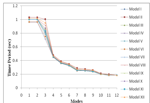
Fig. 20 Comparison of Time Period for different models without window opening
