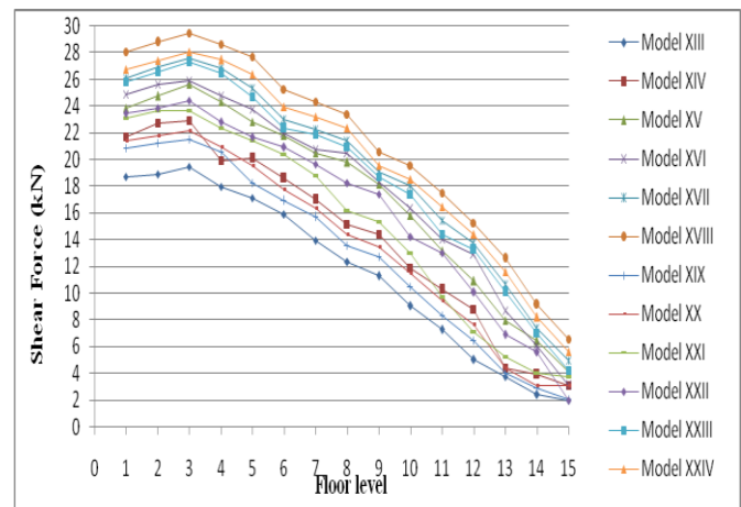
Fig. 24 Comparison of Shear Force for different models with window opening
