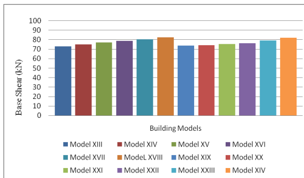
Fig. 26 Comparison of Base Shear for different models with window opening
