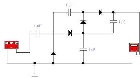
Figure 1. Villard voltage multiplier
