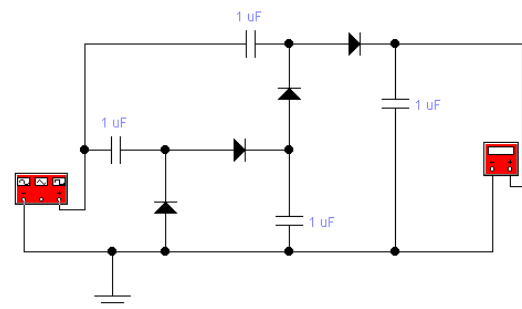
Figure 2. Dickson voltage multiplier circuit
