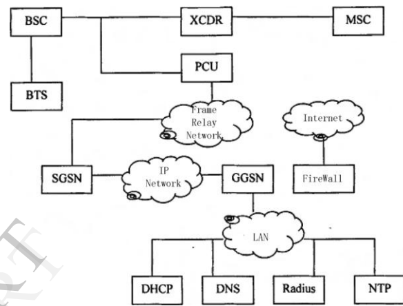
Figure 1. GPRS network structure
