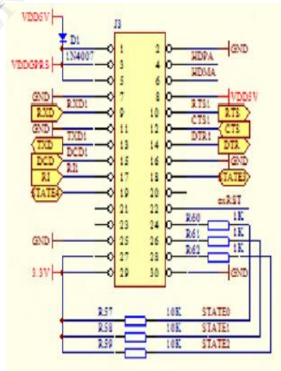
Figure 3. GPRS interface circuit
