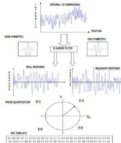
Fig 6.1 An illustration of the feature encoding
