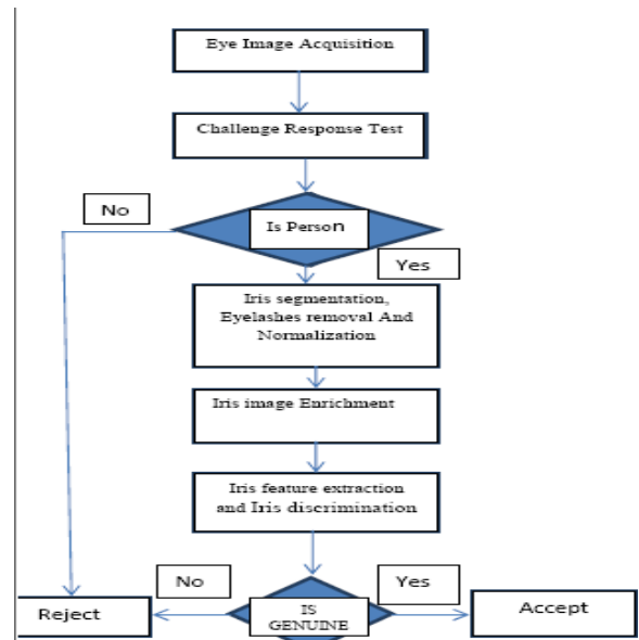
Fig 4.1 Block diagram of the proposed approach
