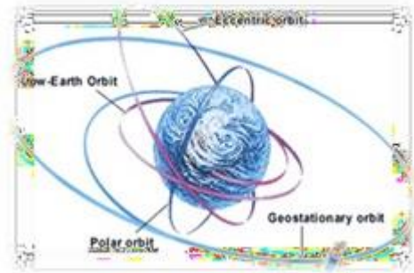
Fig.3 Different Orbits
