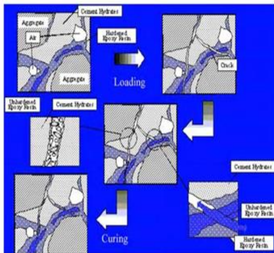
Figure 1 Simplified model for autohealing mechanism of microcracks in epoxy-modified cementitious systems.
