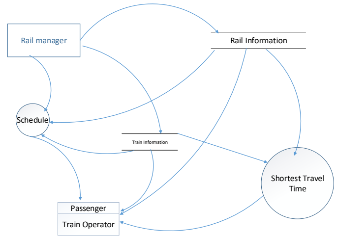
Figure 6: Data flow diagram for the travel time system
