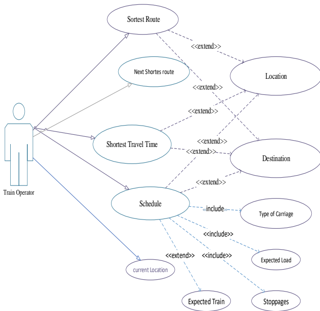
Figure 4: Train Operator Use Case
