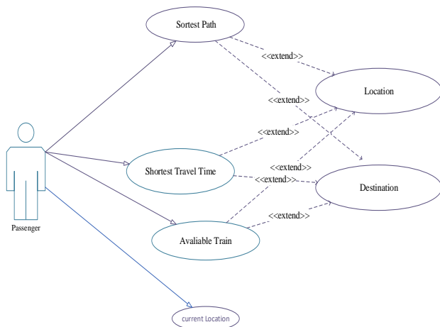
Figure 5: Passenger Use Case
