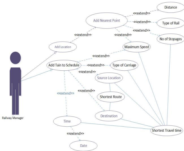
Figure 3: Railway Manager Use Case
