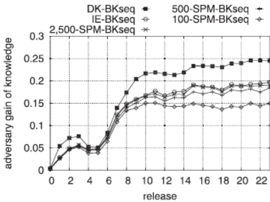
(c) Defense based on SPM-BK^{seq}
