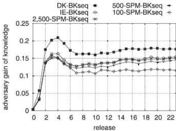
(b) Defense based on IE-BK^{seq}
