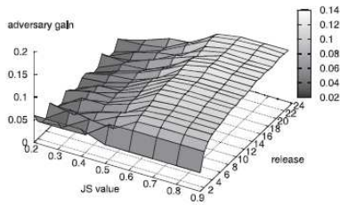
Fig. 7. Adversary gain versus JS divergence ( t = 0.5 ).
