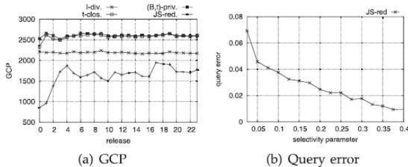
Fig.5. Data quality evaluation
