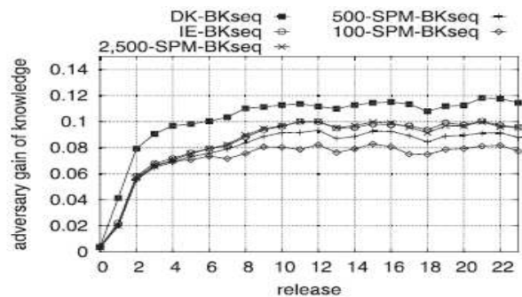
(a) Defense based on DK-BKseq
