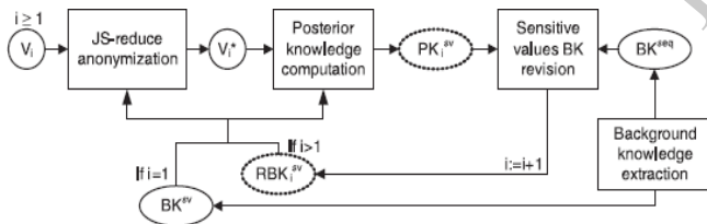
Fig.1. Defense mechanisms.
