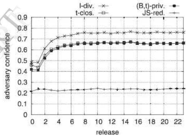
Fig.4. Adversary confidence.
