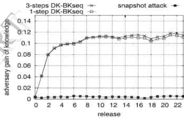
(c) JS-red.
