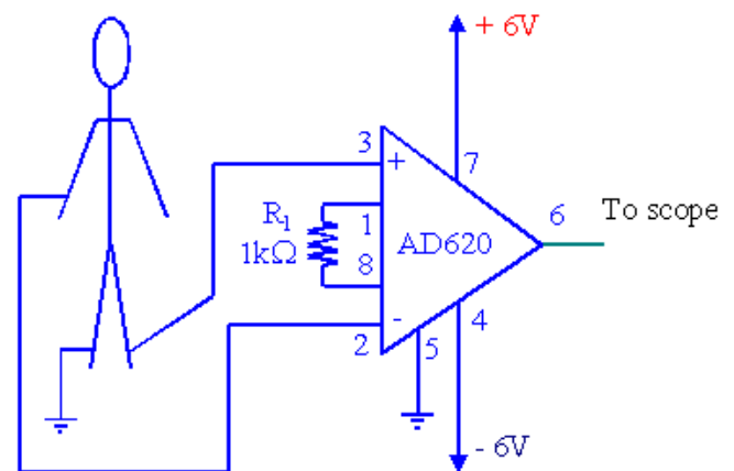
Fig 1: ECG Circuit Diagram
