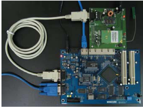
Fig. 4. Communication Unit
