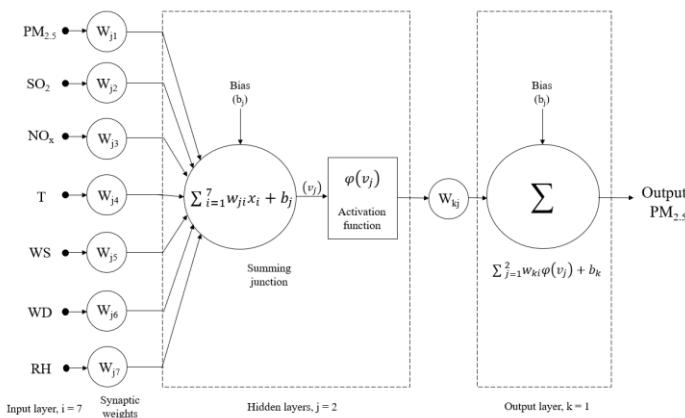
Fig. 4. Schematic network of ANN model
