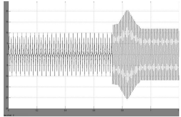
Fig.5.Grid Current
