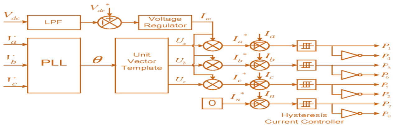
Fig. 3. Block diagram representation of grid-interfacing inverter control
