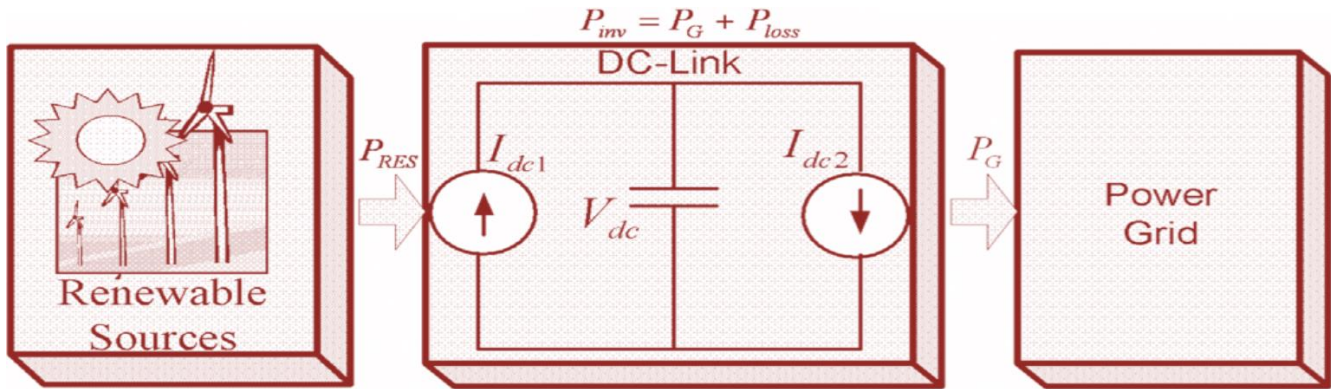
Fig. 2. DC-Link equivalent diagram.
