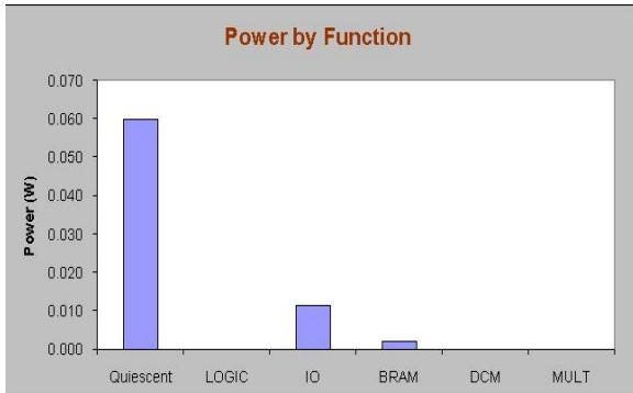
Fig 3- Power analysis of basic memory
