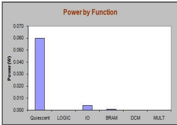
Fig 7- Power analysis of proposed memory
