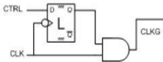
Fig 4 Concept of clock Gating
