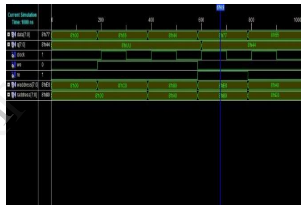
Fig 1- Simulation result of basic memory
