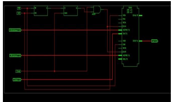
Fig 5- RTL Schematic of proposed memory
