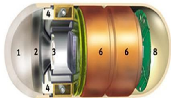
Fig 3.5components of capsule
