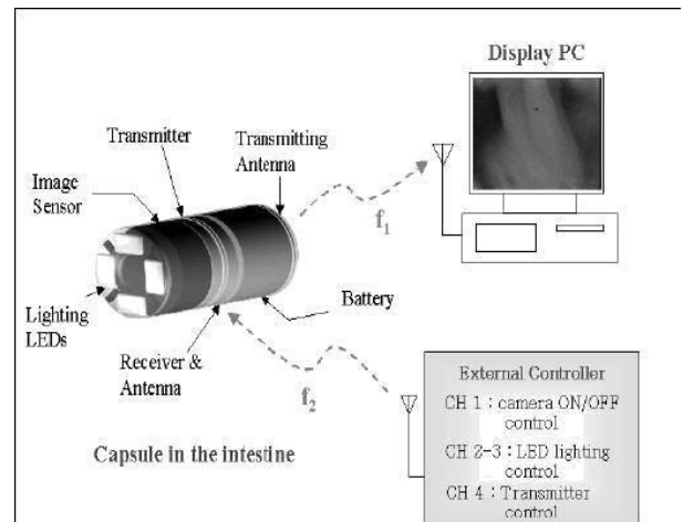
Fig. 1. Conceptual diagram of bi-directional wireless endoscopy system
