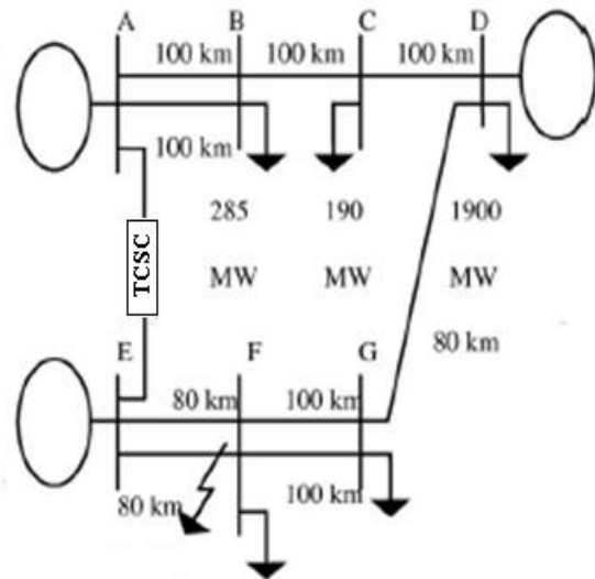
Fig 2.Three machine 7 bus system test system
