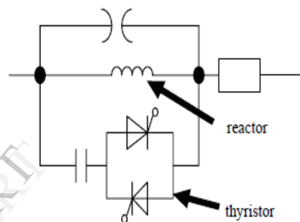
Fig.1 TCSC(Thyristor controlled series compensator) model
