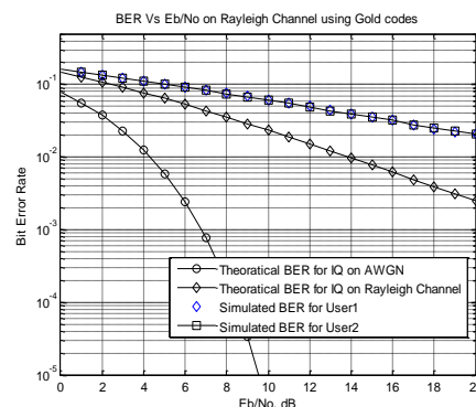
Fig 3 BER Vs E_b/N_0 on Rayleigh Channel using Gold Codes
