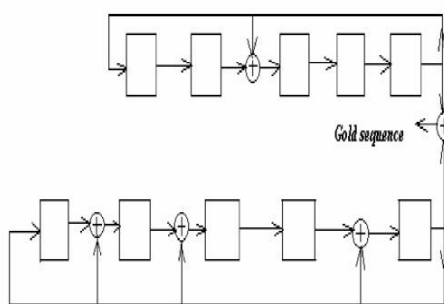
Fig 2: Generation of Gold Code Sequence of length 31
