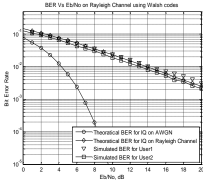
Fig 4 BER Vs E_b/N_0 on Rayleigh Channel using Walsh Codes
