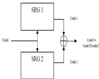
Fig 1: Gold Code Sequence Generator
